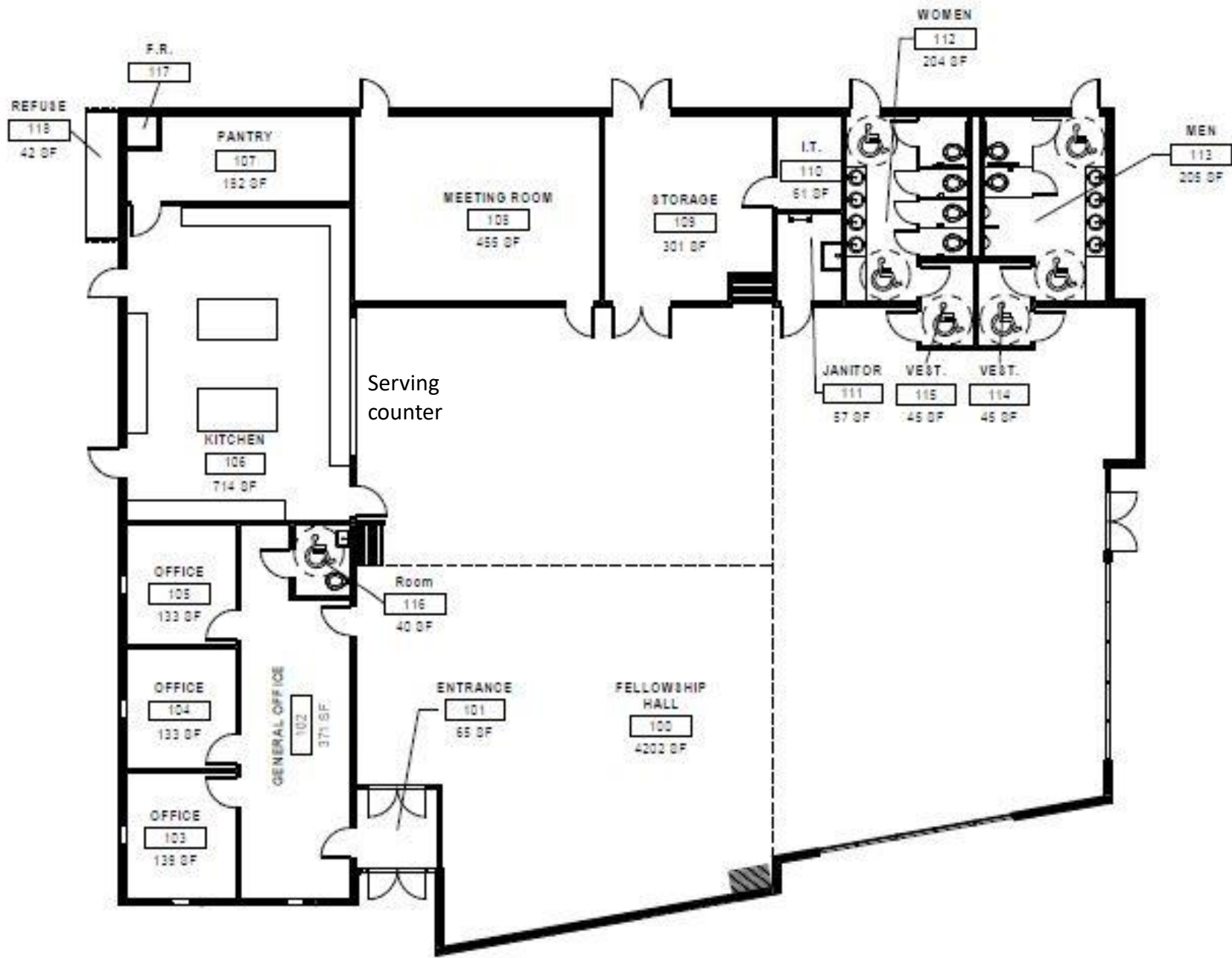
Plan View of Single Story Ministry Center
