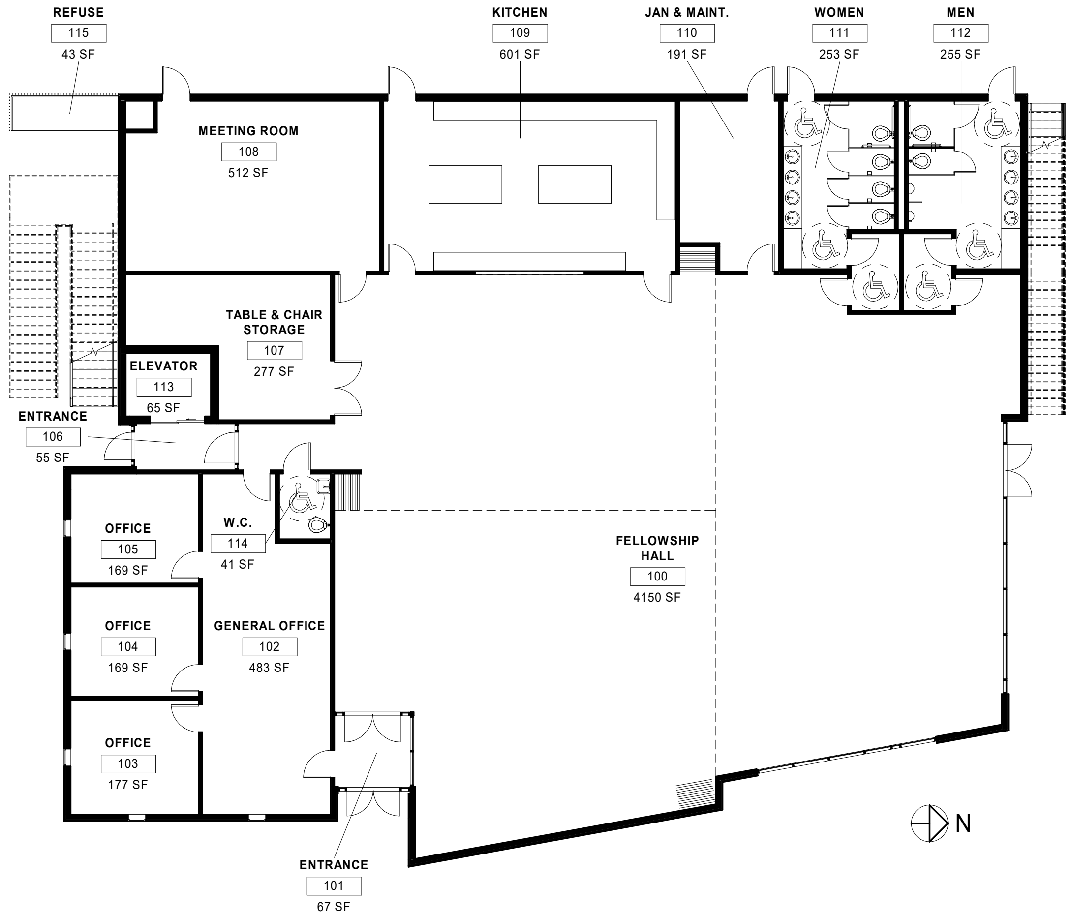
EMMANUEL LUTHERAN FELLOWSHIP BUILDING FLOOR PLAN: 1ST FLOOR
